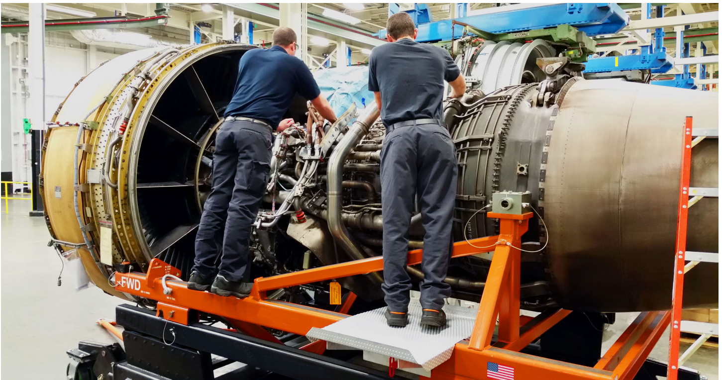
Notice how the technician on the left must lean forward, balanced on the narrow rail on the balls of his feet, while the technician on the LOCKN-WALK stands upright in comfort with a wide working range of movement across the platform.
